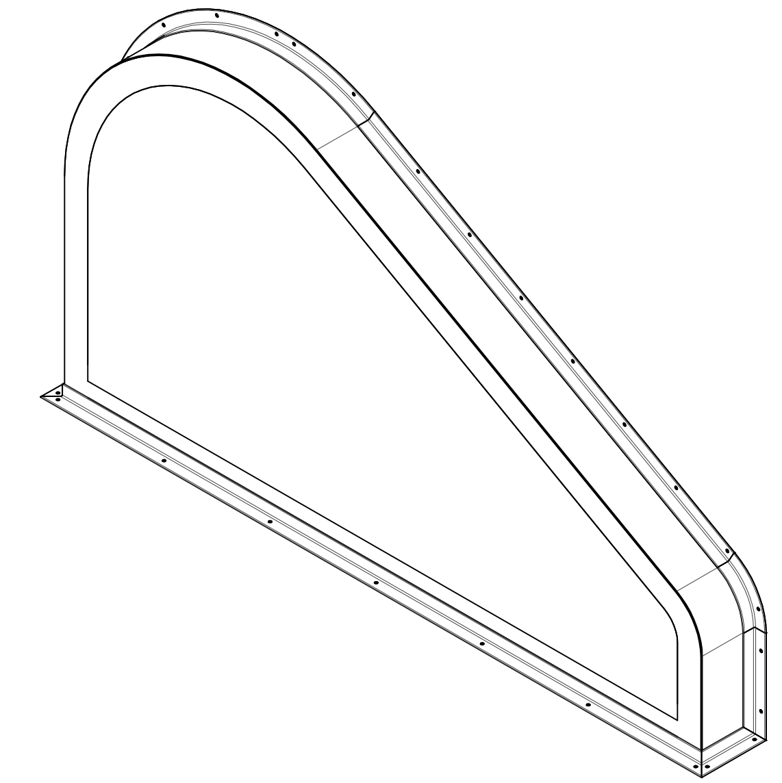
ISOMETRIC VIEW SCALE 3/4"=1'-0"
